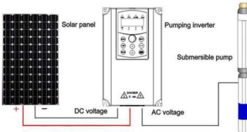
Figure 1 Structure of solar pumping system
