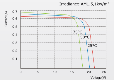
SLP010-12 I-V Curves
