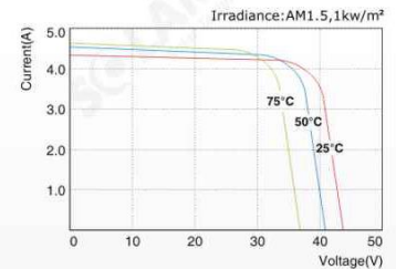
SLP135-12 I-V Curves
